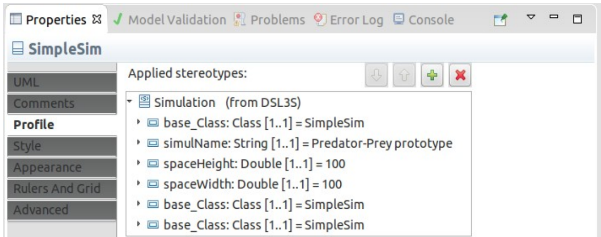
Figure 4 - The Properties view for an element with an applied stereotype. By clicking on a property it is possible to change its value.
